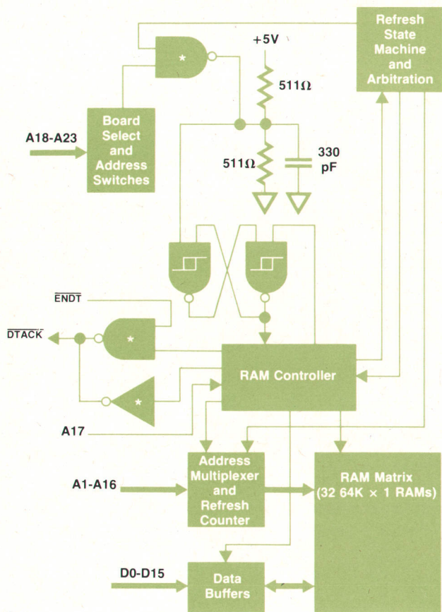
Fig. 7. Block diagram of 256K-byte RAM board.
