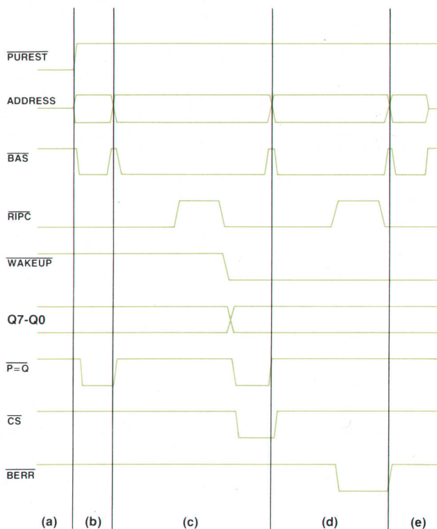
Fig. 6. Timing diagram for autolocating circuitry.
